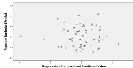
Fig. 2. Distribution graph of regression residuals against predicted values.
